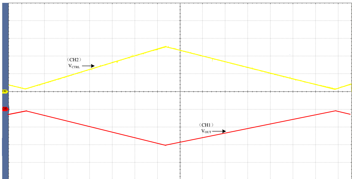
CH1: 2000V/Div CH2: 2V/Div M: 500ms V_CTRL: 0.25V ~ 5V V_OUT: -40V ~ -4000V
